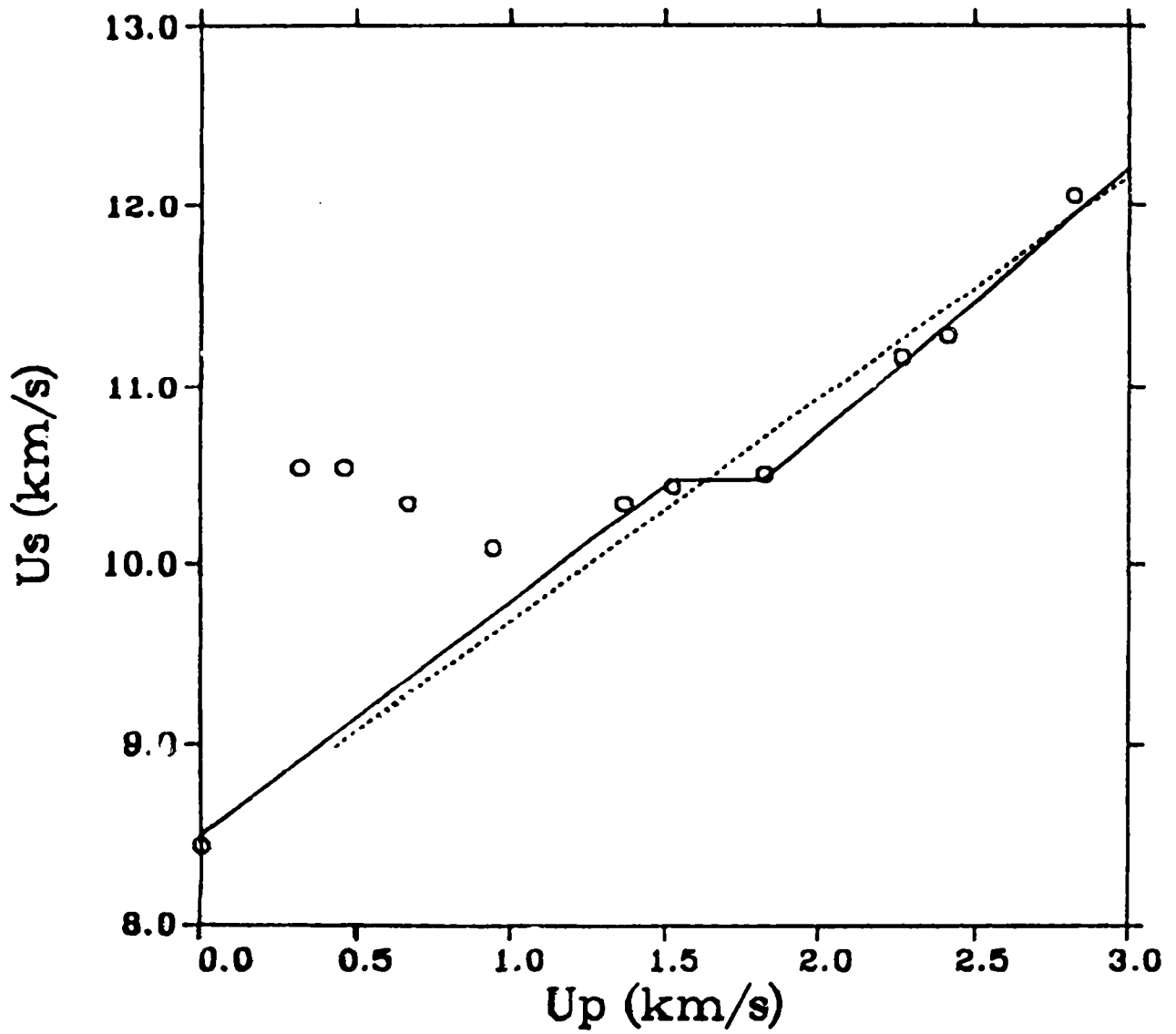
Figure 1. Calculated Hugoniot for material numbers 7611 (solid line) and 7610 (dashed line) compared with experimental data from Ref. 2.
